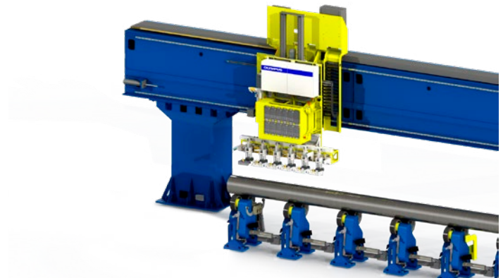
Rotating Tube Inspection System (RTIS)
